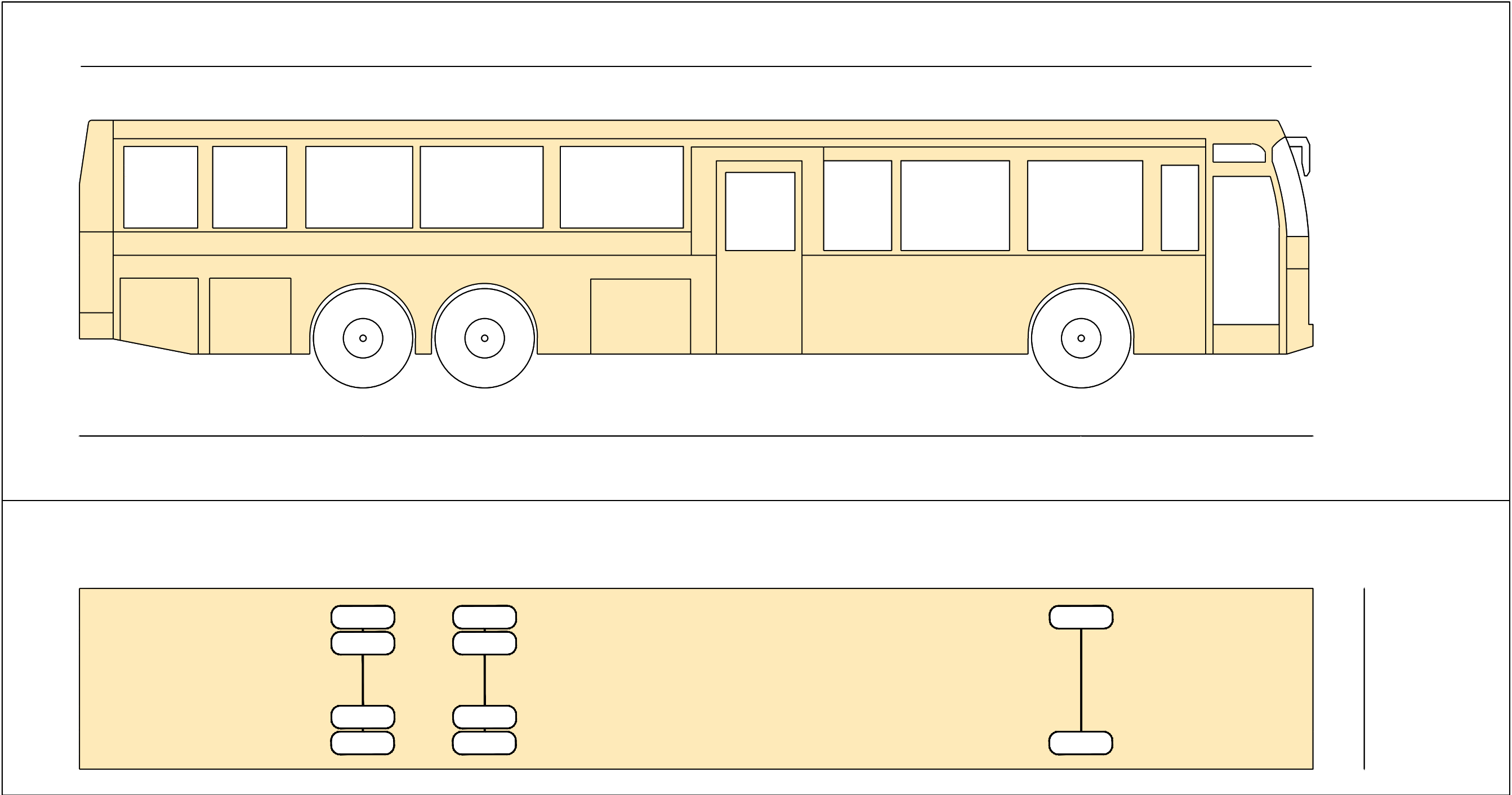
Standard: Norway, Name: 2018 Buss (B), Svv HbN100, Total length: 15.00(m)
